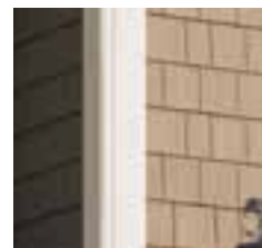
Vinyl Carpentry Beaded SuperCorner and J-channel in colonial white.
